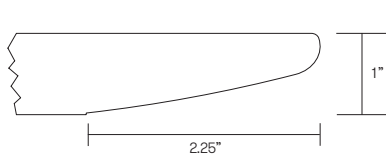
Edge Detail # 38 HPL laminate over a 1” MDF core counter balanced. The edge is cut back with a chamfer. The edge is clear finish as standard or can be stained.
