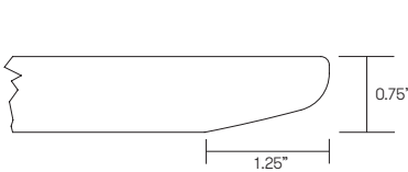
Edge Detail # 43 0.75” solid wood.
