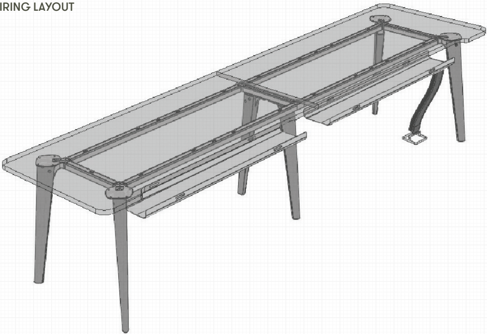
PAILO INLINE DESKS TYPICAL WIRING LAYOUT
