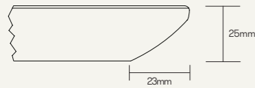
Ref Group Number 28 25mm MDF core, specified laminate face & counterbalance with 23mm chamfered edge. The edge is clear finish as standard or can be stained.
