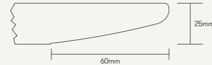
Ref Group Number 38 25mm MDF core, specified laminate face & counterbalance with 60mm chamfered edge. The edge is clear finish as standard or can be stained.
