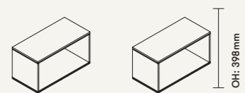
CCRT2BPCB - 2 Bay Ply Closed Box OW: 840mm OD: 410mm CRT2BMCB - 2 Bay MFC Closed Box OW: 840mm OD: 410mm
