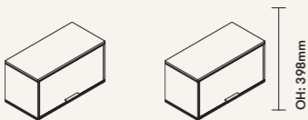
CRT2BPFDB - 2 Bay Ply Box with Flipper Door OW: 840mm OD: 392mm CRT2BMFDB - 2 Bay MFC Box with Flipper Door OW: 840mm OD: 392mm
