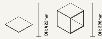
CRTPS - Ply shelf OW: 422mm OD: 12mm
